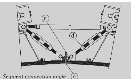
Segment connection angle (c)
