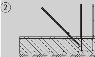
Screwing in the tie rod
