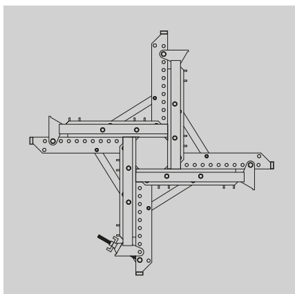
Both rectangular and square sections can be formed from 20x20 cm to 60x60 cm in 5 cm steps
