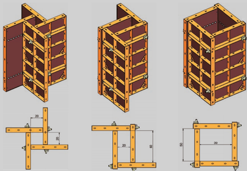
With four elements each square and rectangular column cross-sections can be formed in the adjustment range of 20 cm to 50 cm in increments of 5 cm.
