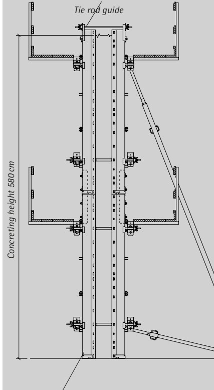
Segment 240x300 cm, with extension segment 240x300 cm
