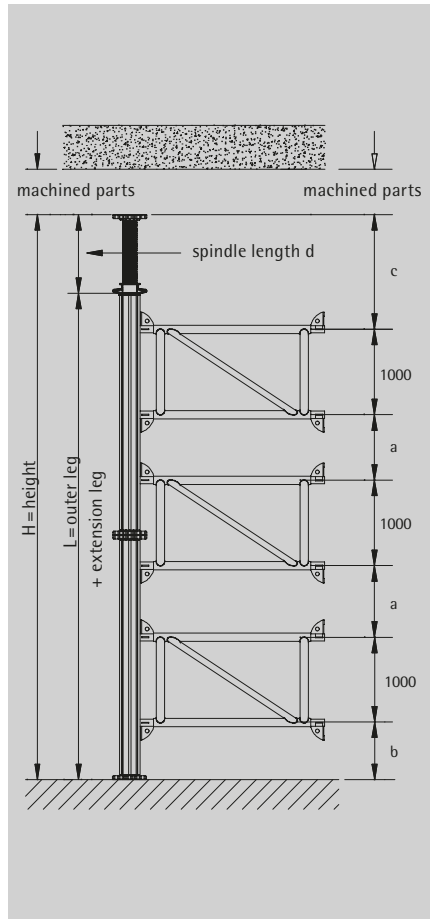
Detail: Short link 400
