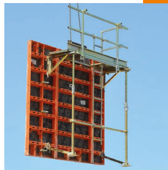
Moving the formwork with Multip
