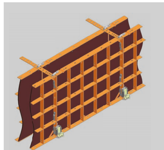
mount the perforated ties at every panel joint adm. load: 10 kN
