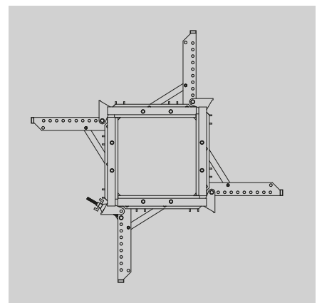
Both rectangular and square sections can be formed from 20x20 cm to 60x60 cm in 5 cm steps
