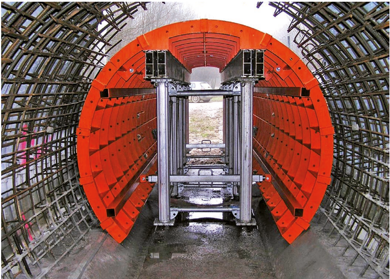
Formwork carriage – foldable formwork with GASS shoring system
