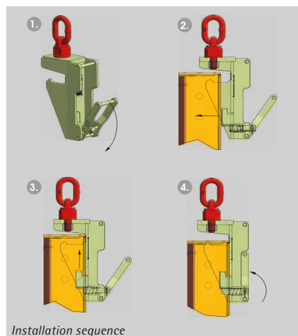
Installation sequence
