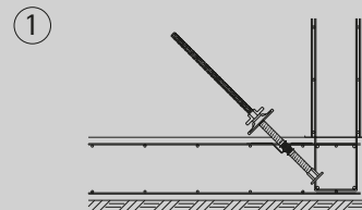
Fitting the V-guide DW26,5 with tie rod, concreting
