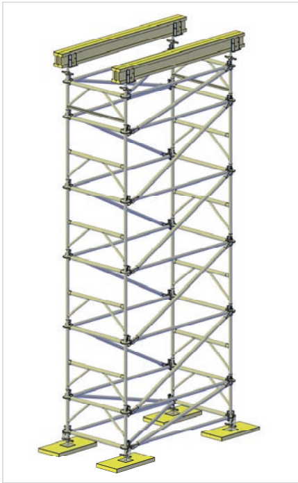
Shoring tower TG 60
