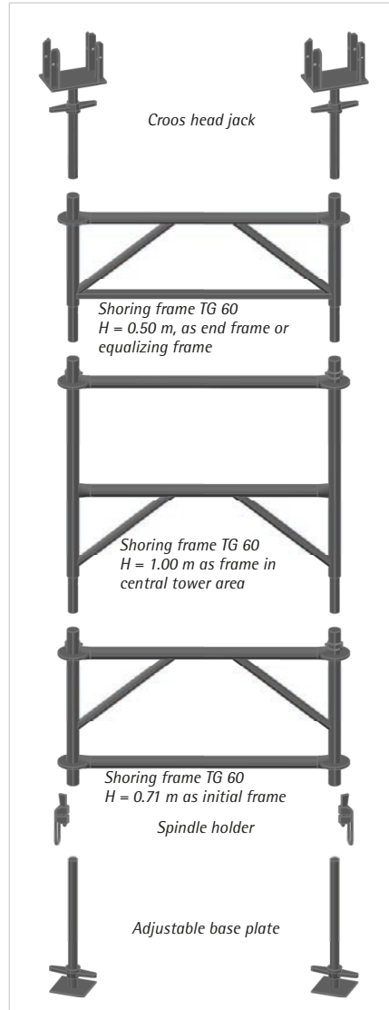
Basic components of the TG 60 shoring tower
