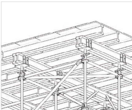
Support beam and cross-beam
