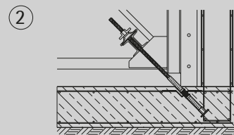
Assembling the formwork, supporting jack and waler
