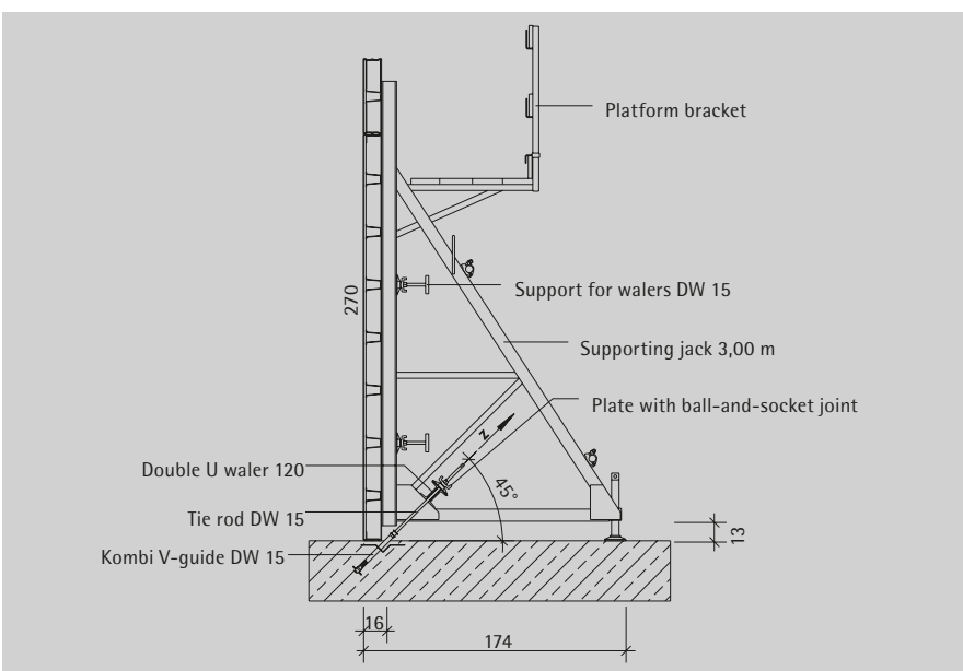
Assembling the formwork, supporting jack and waler
