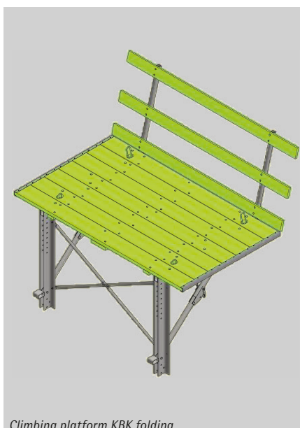
Climbing platform KBK folding
