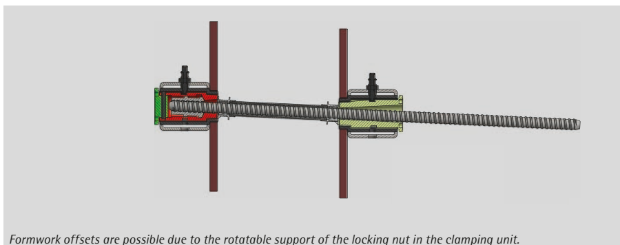
Formwork offsets are possible due to the rotatable support of the locking nut in the clamping unit.
