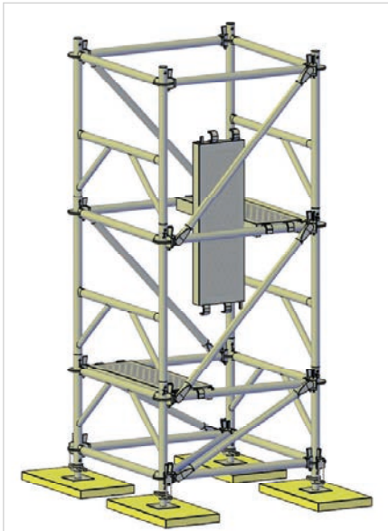
Repositioning the assembly decks
