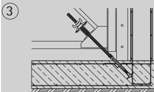
Assembling the formwork, supporting jack and waler
