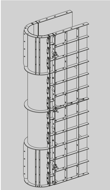
Circular column half circles with Modular formwork.
