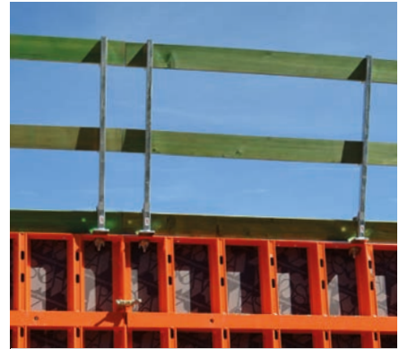
Secuset with wooden boards on LOGO.3 formwork
