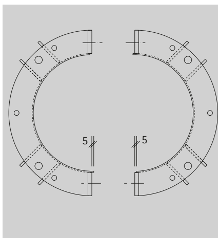
A 5 mm wide overlap of the steel faced plywood compared to the frame prevents any concrete from bleeding out of the joint of the half circles.
