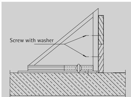
Conventional formwork with planks
