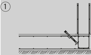
Fitting the kombi V-guide, concreting
