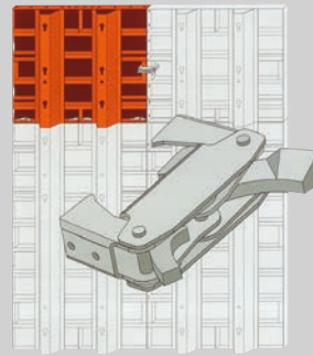
GE panel 200x275 cm
