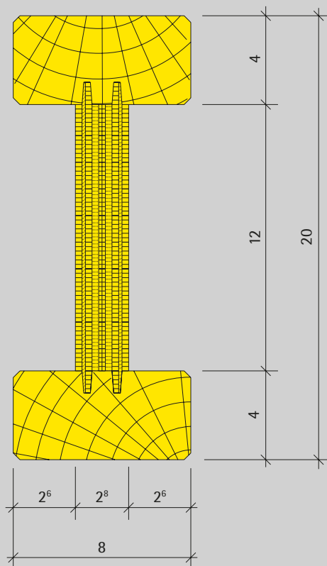
H 20 girder
