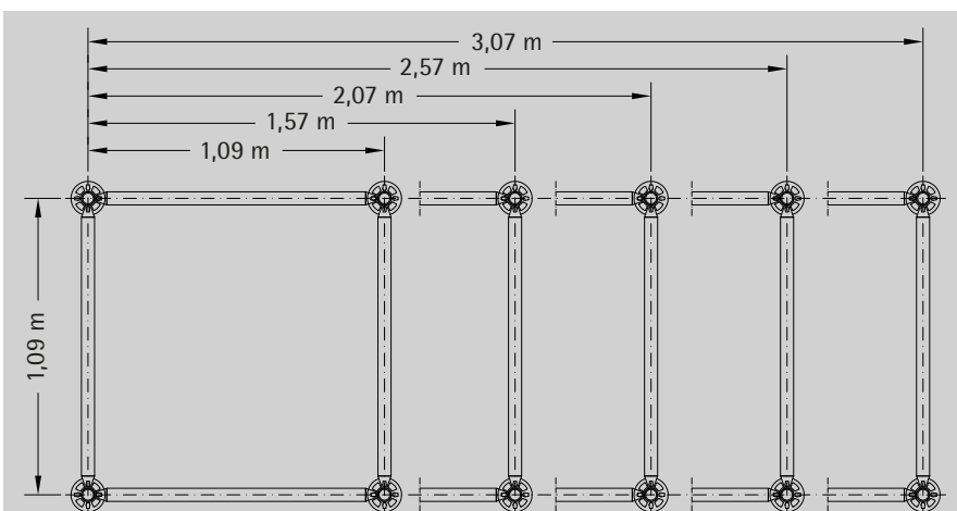
Shoring tower TG 60 - different base layouts
