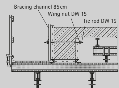
Edgebeam with slab
