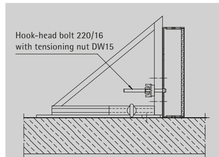
Formwork with steel frame elements lying down (e.g. LOGO, Modular)
