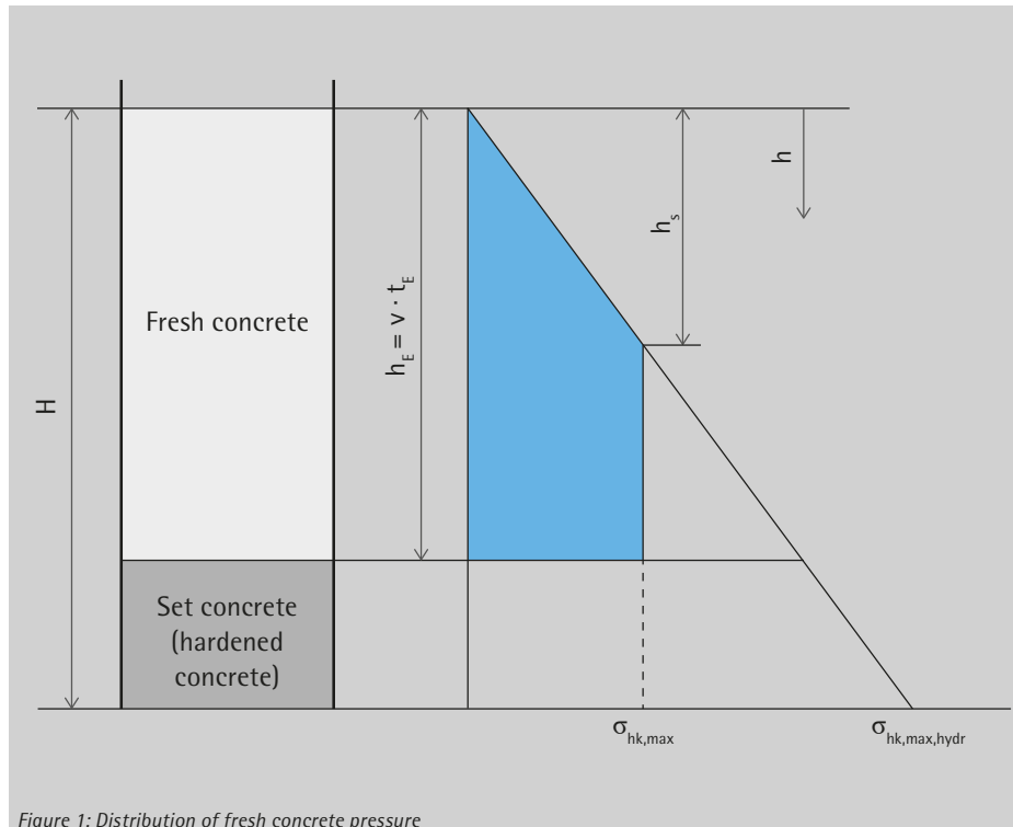
Figure 1: Distribution of fresh concrete pressure
