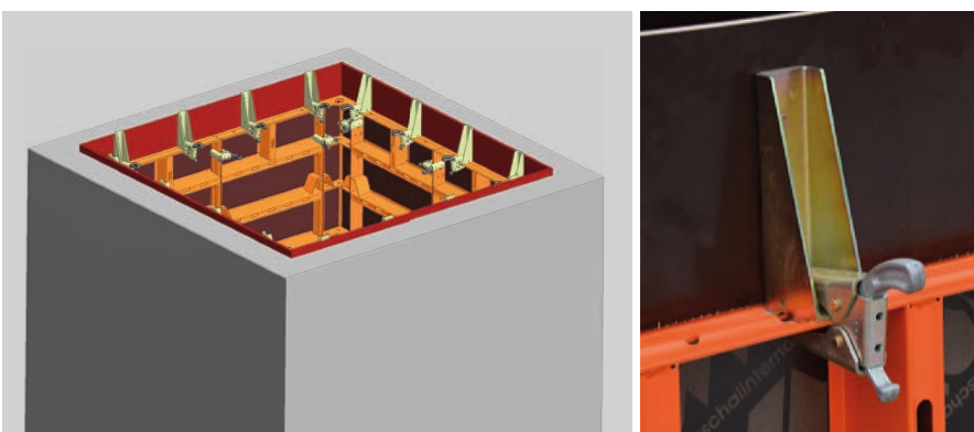
Simple assembly on the upper panel frame of LOGO.3 panels with the wedge clamp.
