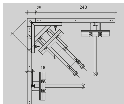
Main-line drawing for using the corner waler.
