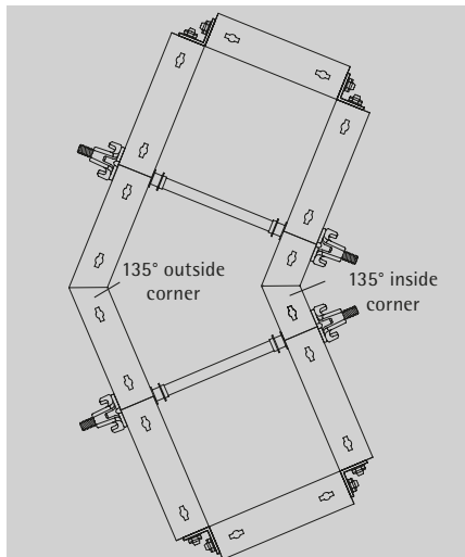
Angle column consisting of Modular panels and rigid 135° corners, suitable formed without expensive special formwork.
