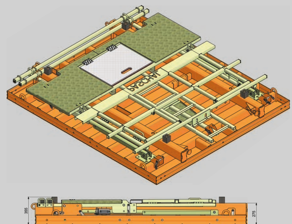
Folded together the panels are a compact unit with a fixed multi-functional working platform "Multipl".
