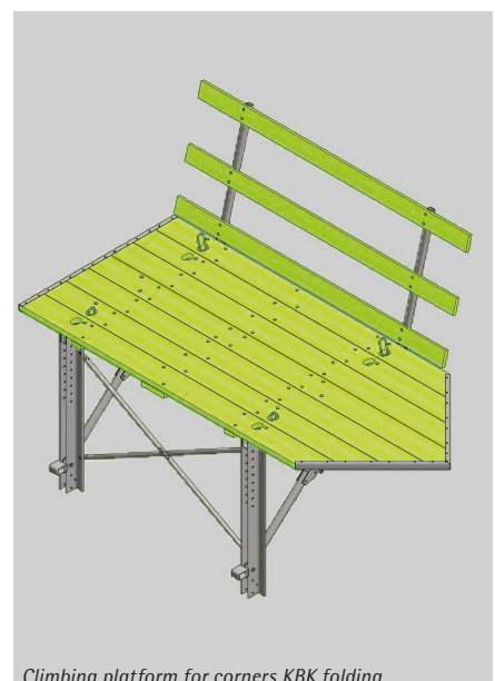
Climbing platform for corners KBK folding
